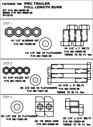
(1) Fastener Kit, PWC Trailer Bunk P/N 001-16030-00
