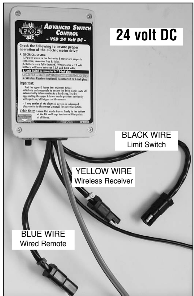
Fig. 4 Advanced Switch Control (ASC). Top image is a 24 volt DC powered unit.
