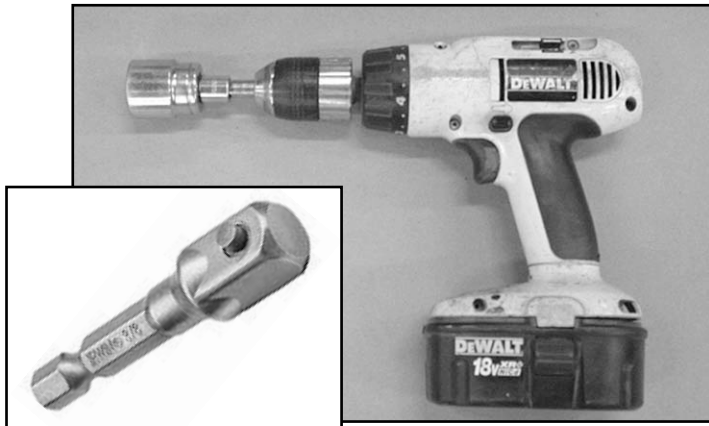
Fig. 26 Cordless Drill with Socket Attachment
