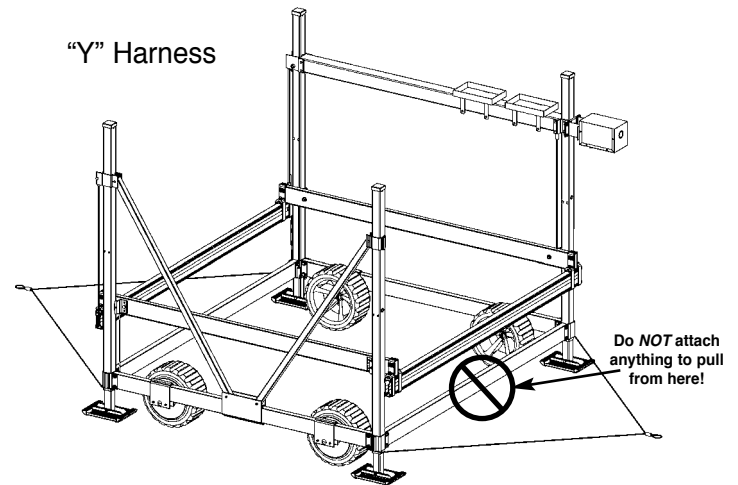
Fig. 33 Proper Pressure Distribution on Lift Frame Using "Y" Cable Harness Set-Up
