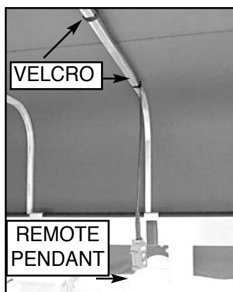
Fig. 17 Velcro One-Wrap
