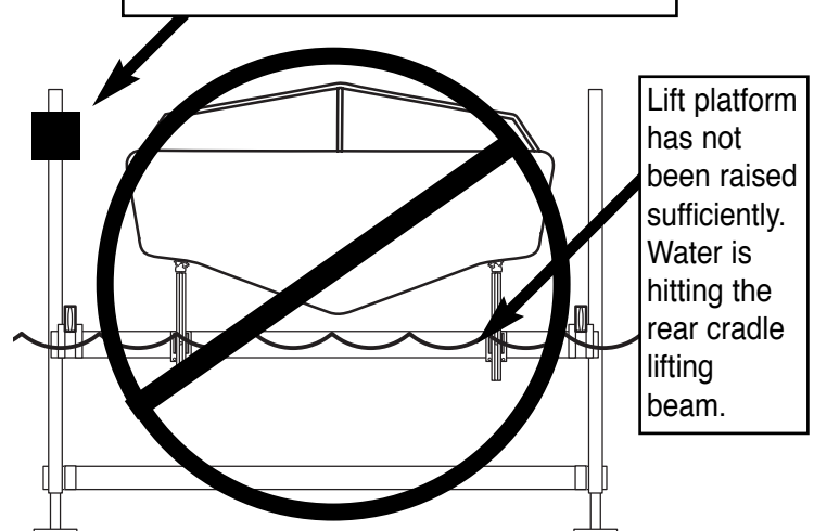
Fig. 14b Do not let cradle lift beam act as a wave-break!
