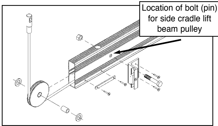
Fig. 64 Side Cradle Lift Beam Pulleys
