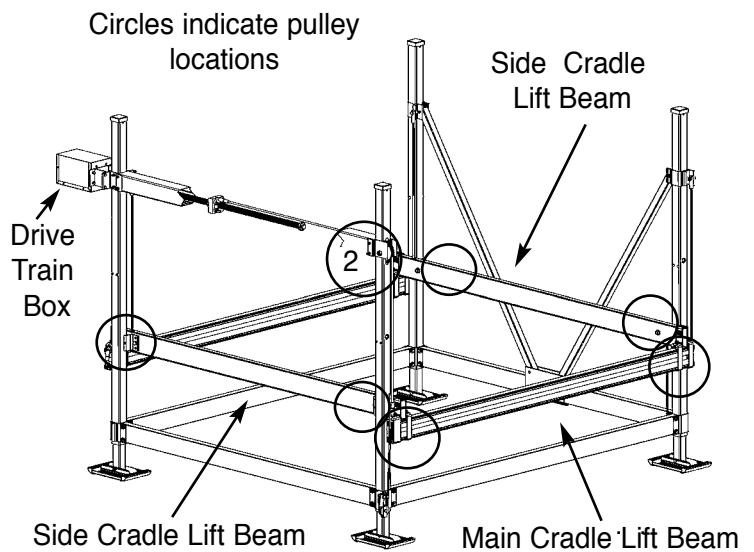
Fig. 65 Location of Eight Sheaves
