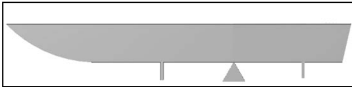
Illustration B: shows the boats center of gravity (CG) centered between the two main lift beams the fact that each of the lift beams is supporting the same amount of weight.
