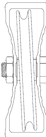
Fig. 63 Pulley with too much side-to-side play (not vertically aligned)
