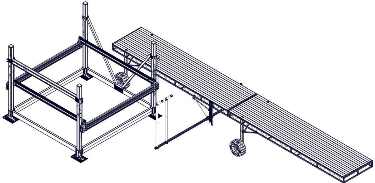
STANDARD CONFIGURATION, CORNER POSTS A & D ARE ON THE SIDE FACING THE BOW FLEX
